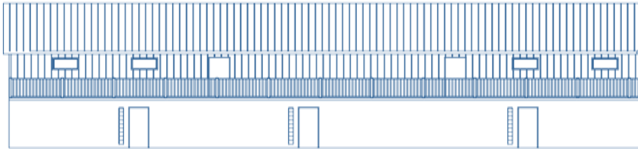
SOUTH ELEVATION
